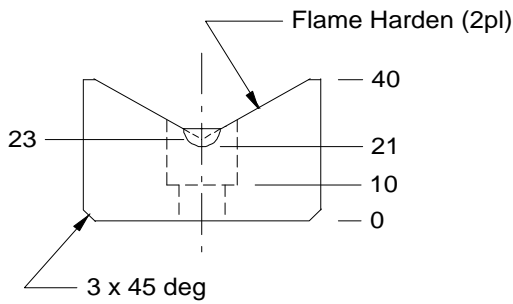
U-Block Profile
